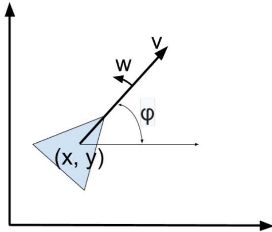
Fig. 2. TurtleBot2 and Unicycle Model
